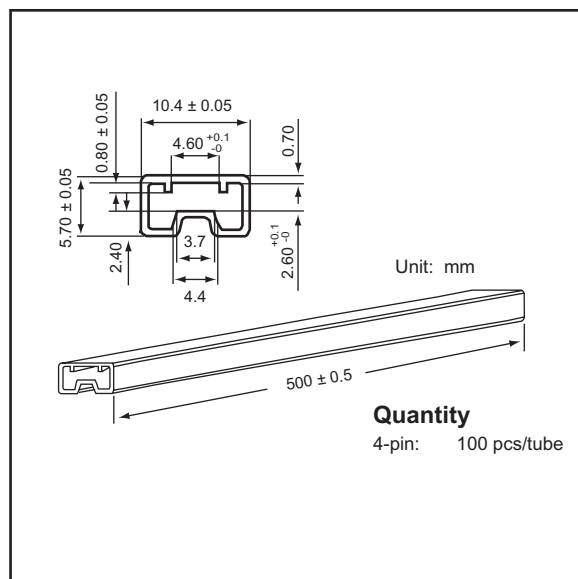
SOP 4-pin
