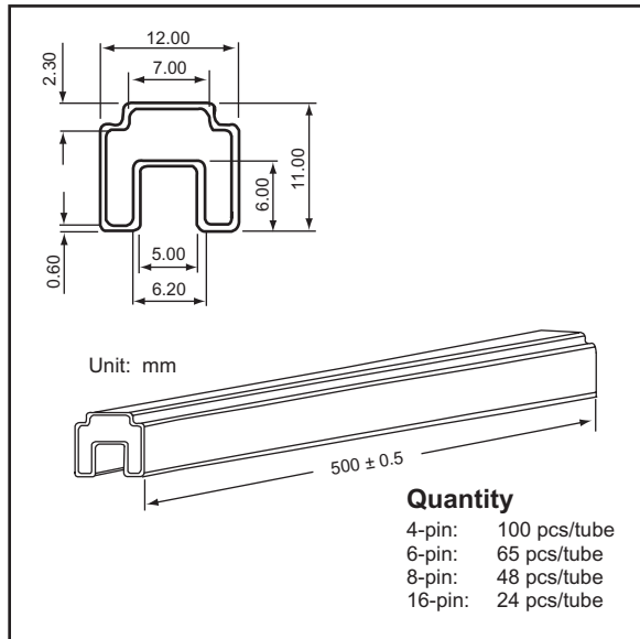
DIP 4, 6, 8, 16-pin
