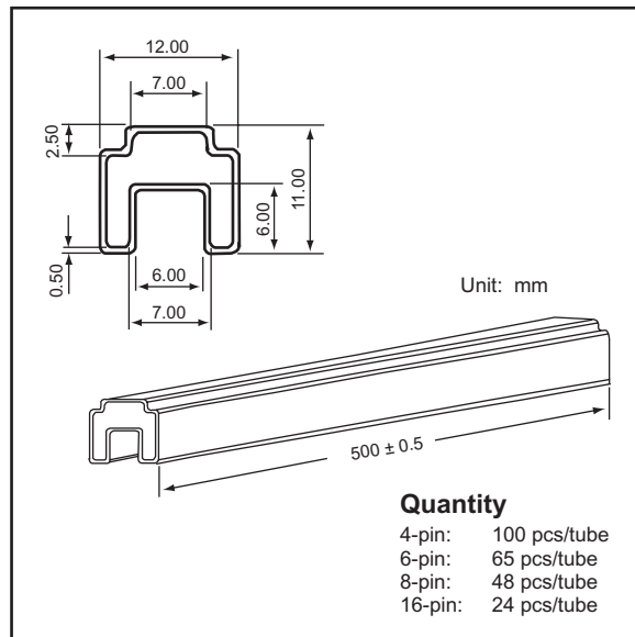
SMD 4, 6, 8, 16-pin
